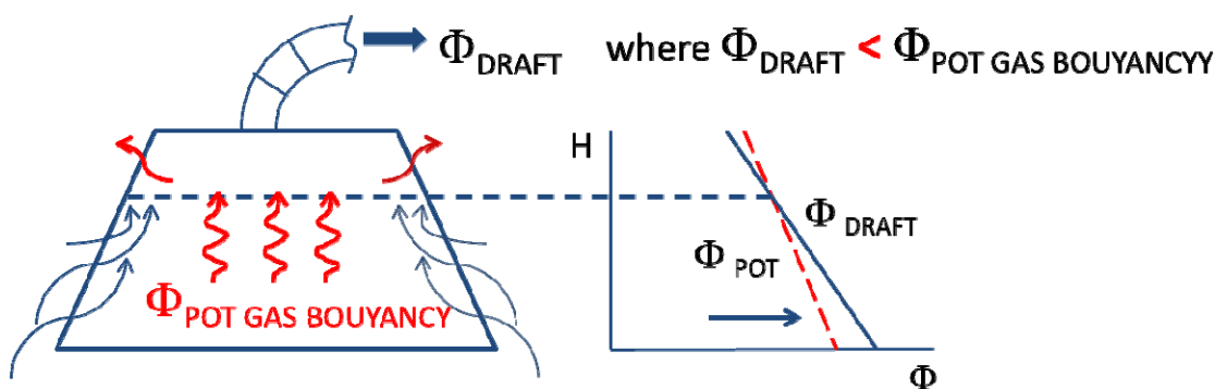
Figure 2. Effect of amperage creep on gas flow.
