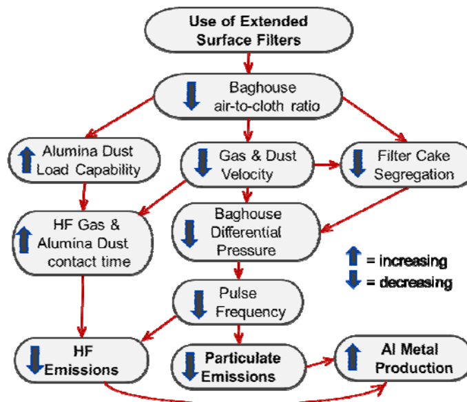
Figure 4. Effect of extended surface filter elements on GTC operation [2].
